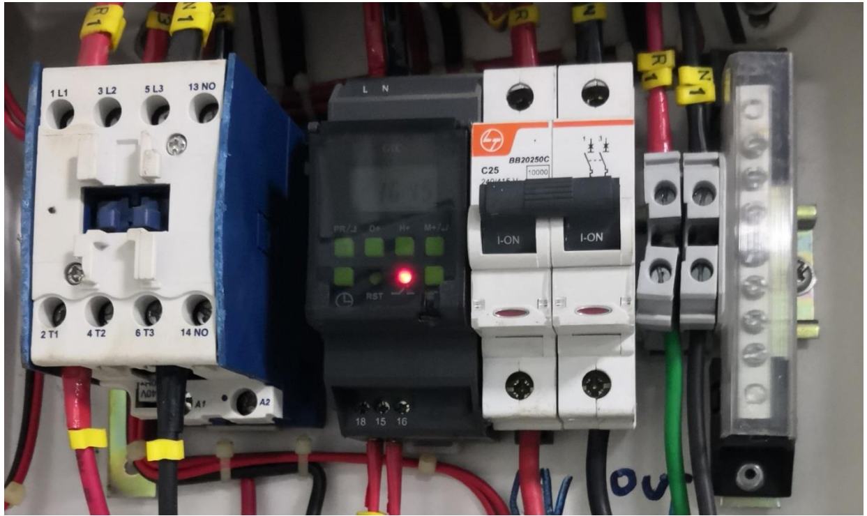
Photograph of sensor based energy conservation system that switches off AC at a defined time.
